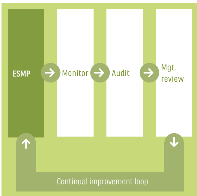
Figure 4. Implementation phase
