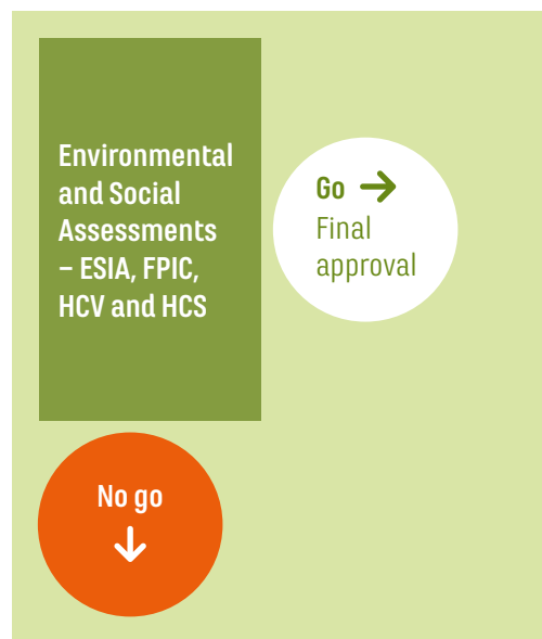
Figure 3. Planning phase
